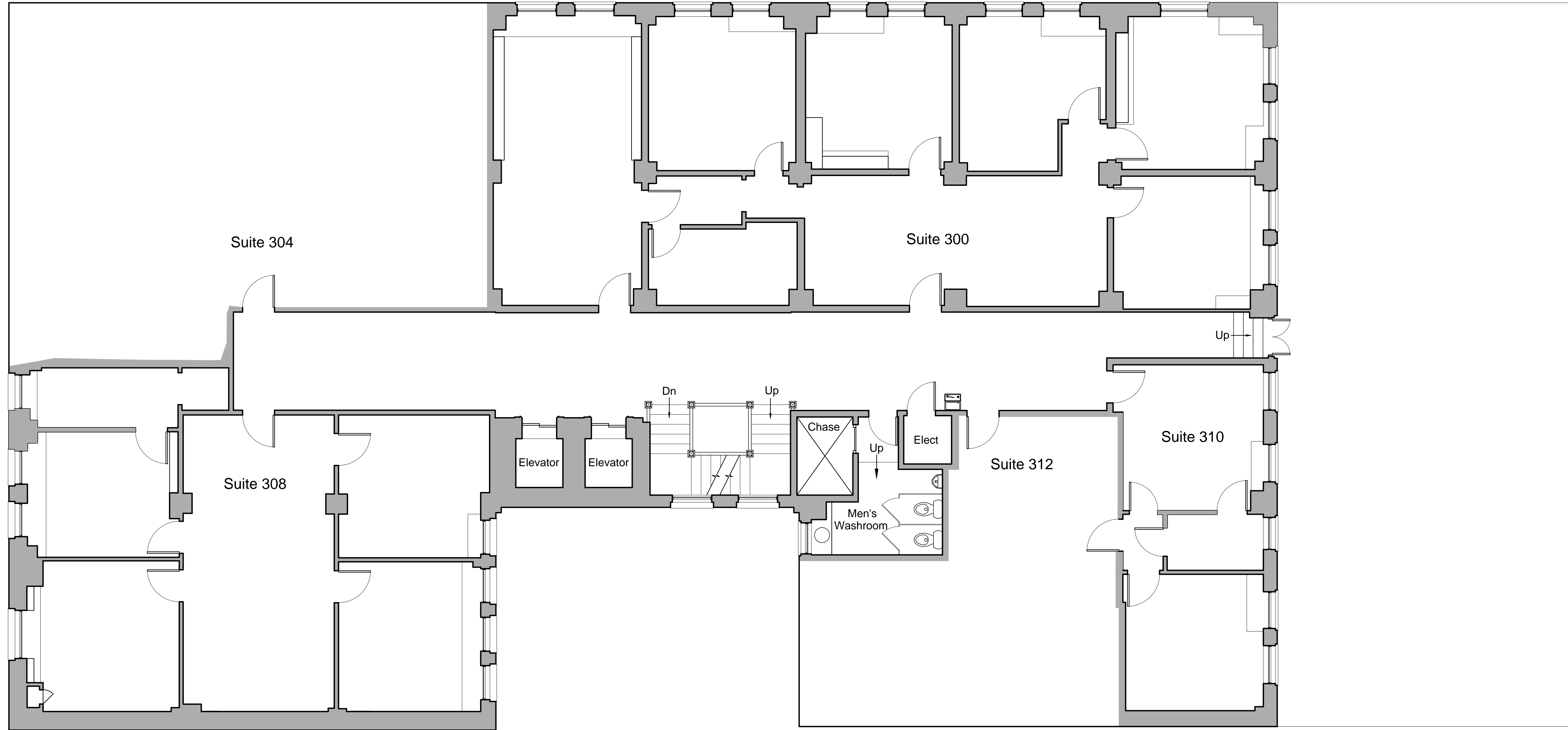
THIRD FLOOR PLAN
